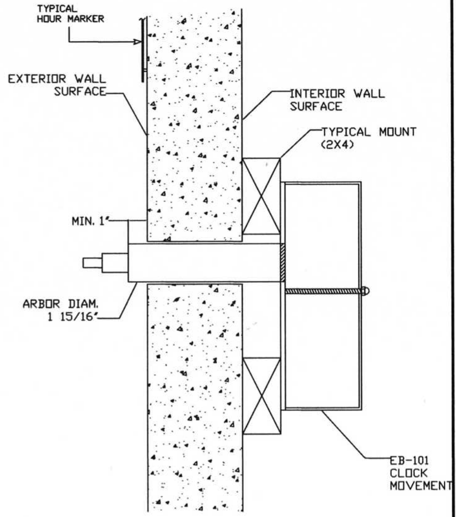
SECTION THRU CLOCK
